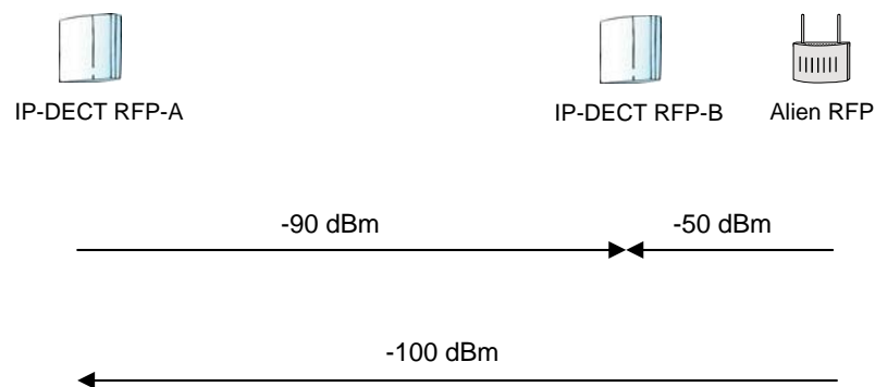
Figure 18. Impact on air synchronization
