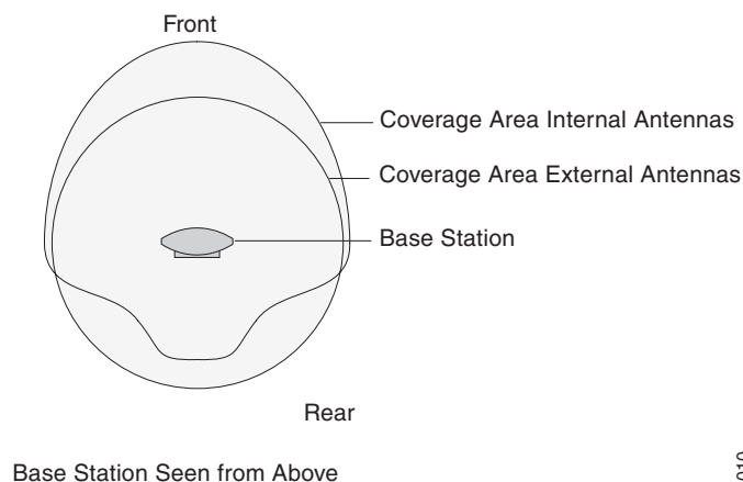
Figure 14. Antenna pattern of the Internal and External Antennas
