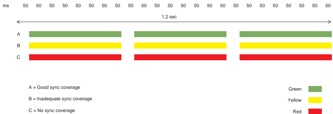
Figure 11. LED2 deployment indications on IPBS1.
