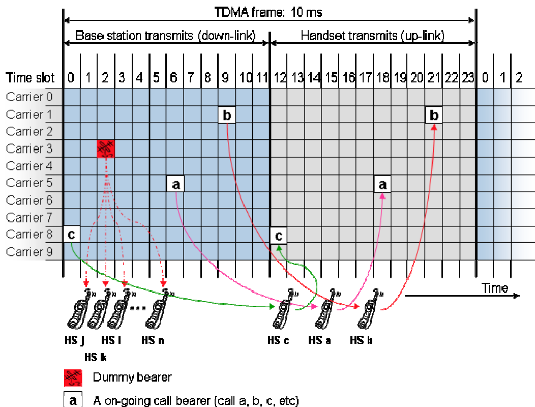
Figure 17. System with three on-going traffic or data calls.
