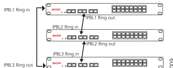
Figure 6. Redundant synchronization
